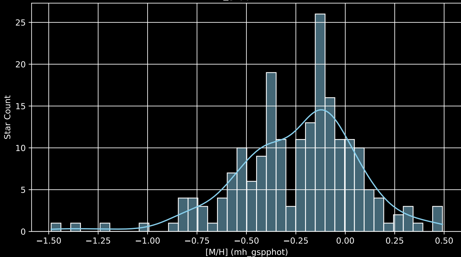
APOGEE DR17 Field: [187-40_MGA [M/H] (mh_gspphot) (n= 203)
