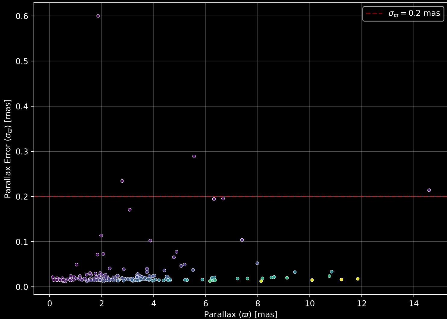
APOGEE DR17 Field: [187-40_MGA] Parallax Quality (n= 205)
