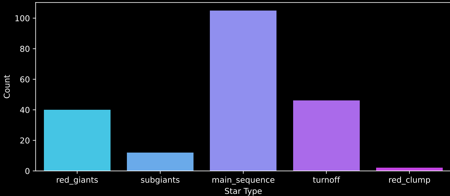
APOGEE DR17 Field: [187-40_MGA] Count plot of Star Type
