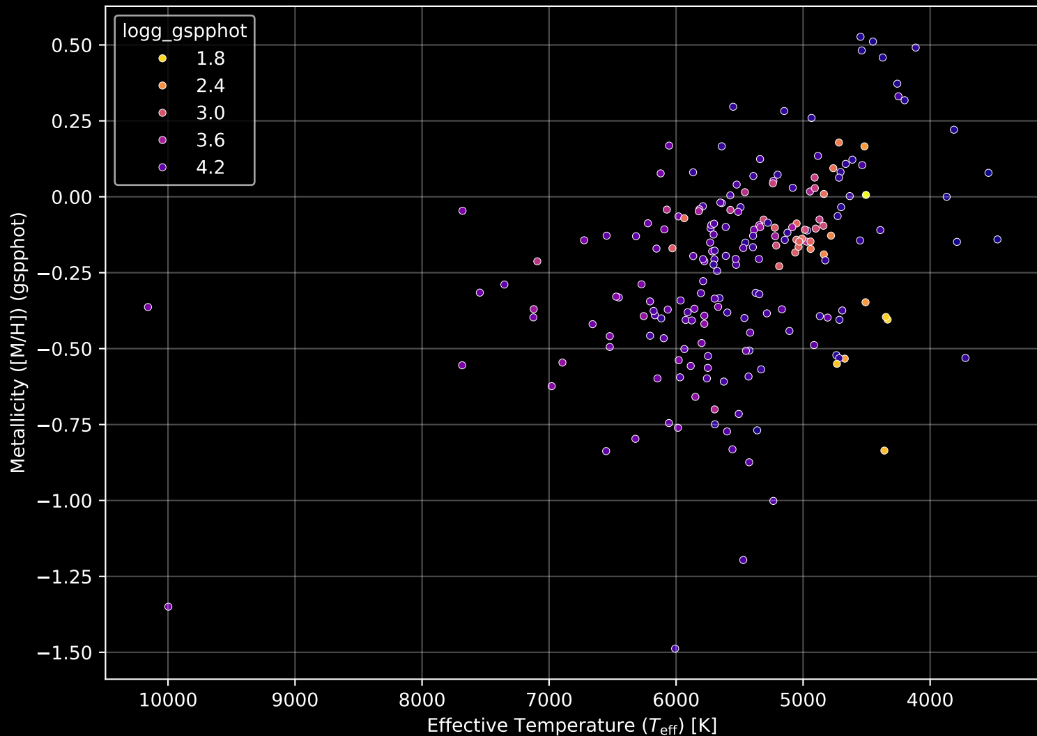
APOGEE DR17 Field: [187-40_MGA] Stellar Population Parameters (n= 205)
