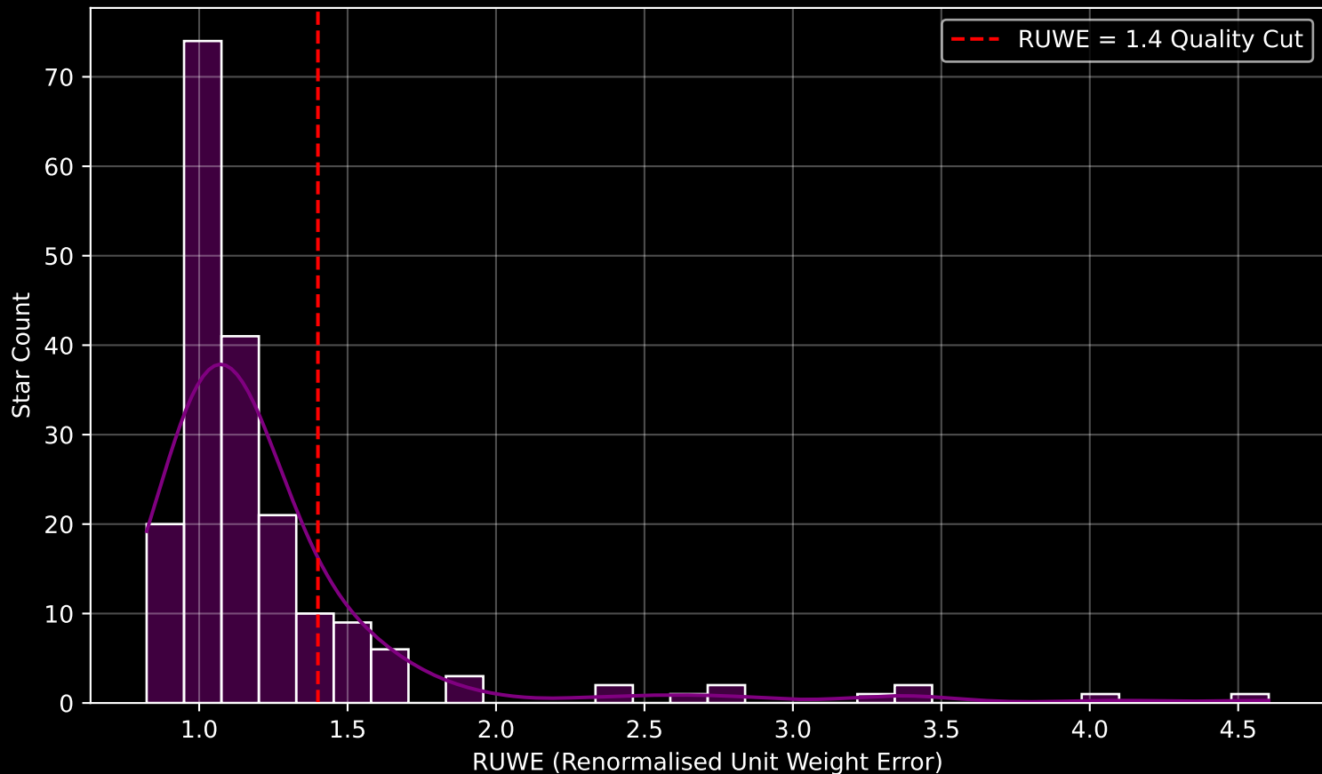
GAPOGEE DR17 Field [187-40_MGA] RUWE Distribution (n= 194)
