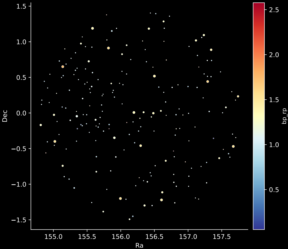
APOGEE DR17 Field: [187-40_MGA] Stars: 205
