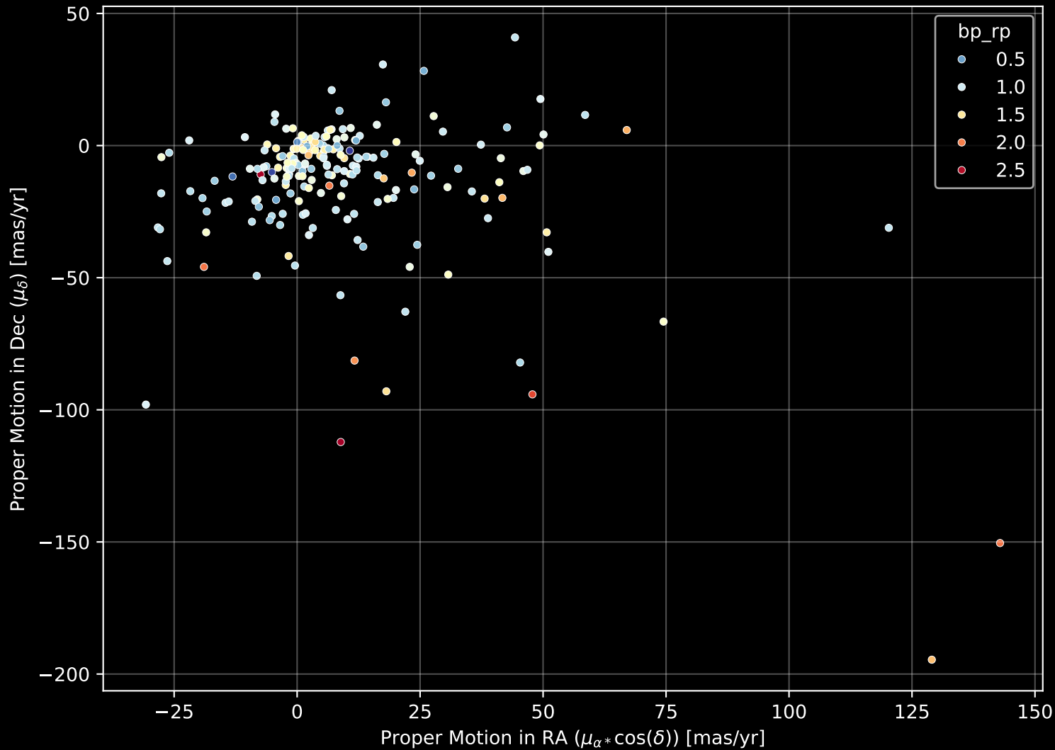
APOGEE DR17 Field: [187-40_MGA] Proper Motion Diagram (n= 205)
